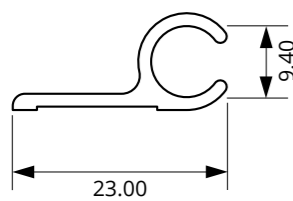
SECTION No. 29-12002 0.228 kg/m
